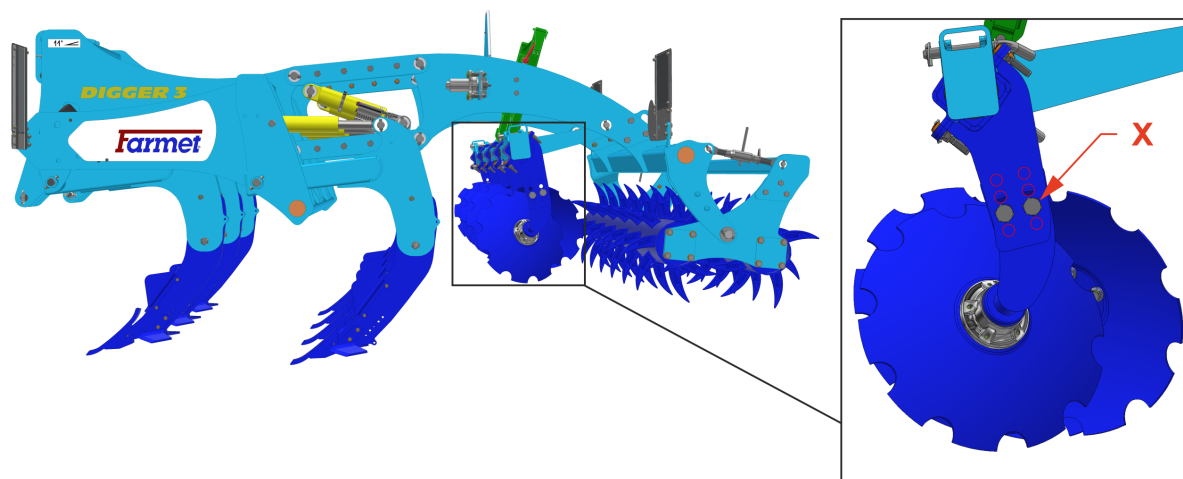
Fig. 7 - Height-adjustable edge leveling discs
