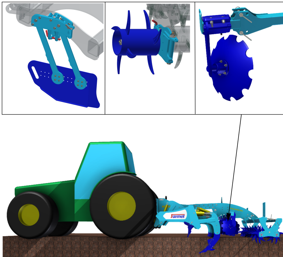
Fig. 3 - working position of the machine
