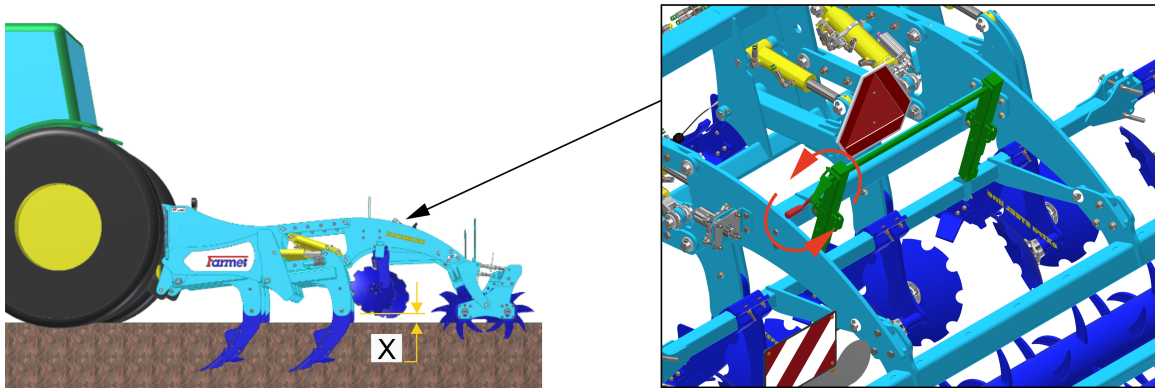
Fig. 5 - setting of the disc height
