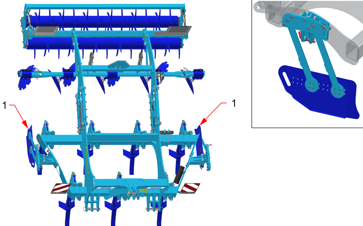
1 – Side deflectors
