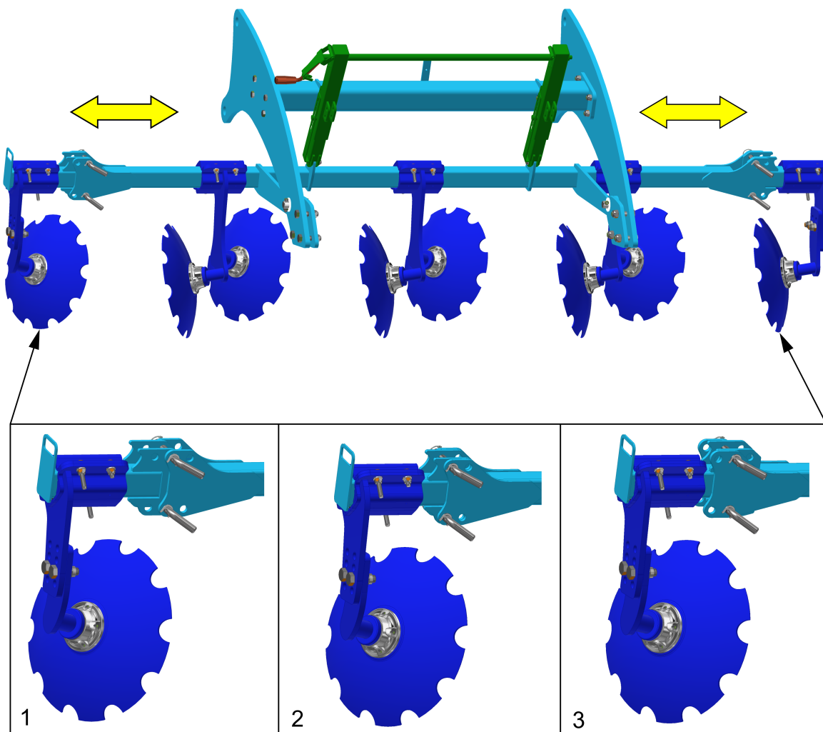
Fig. 7 - Height-adjustable edge leveling discs
