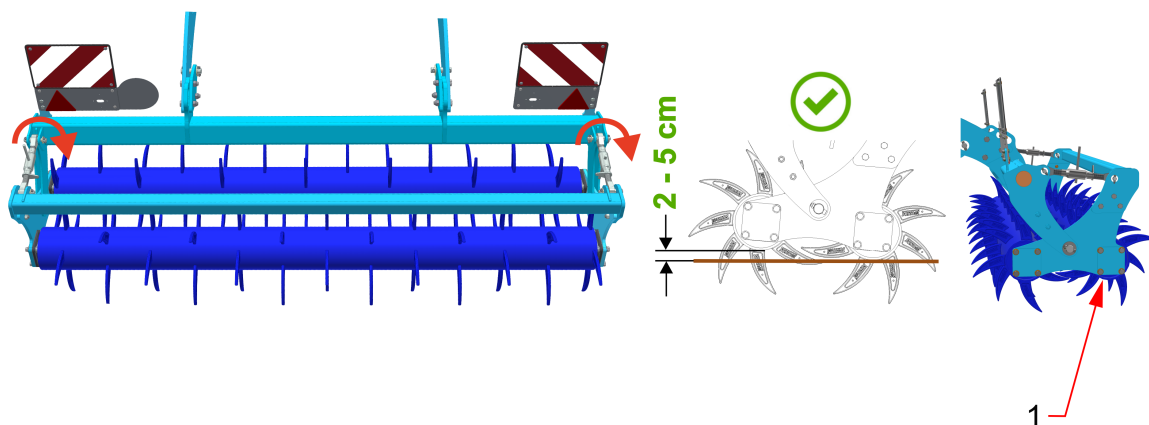
Fig. 8 - roller inclination change
