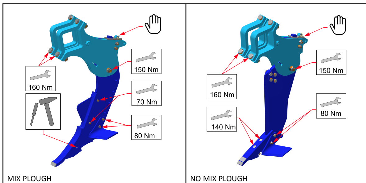
Fig. 9 - replacement of wearing parts of the ploughshare
