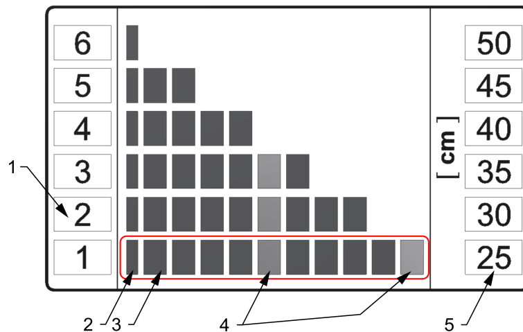
Fig. 4 - washer combinations for the setting of the required depth
